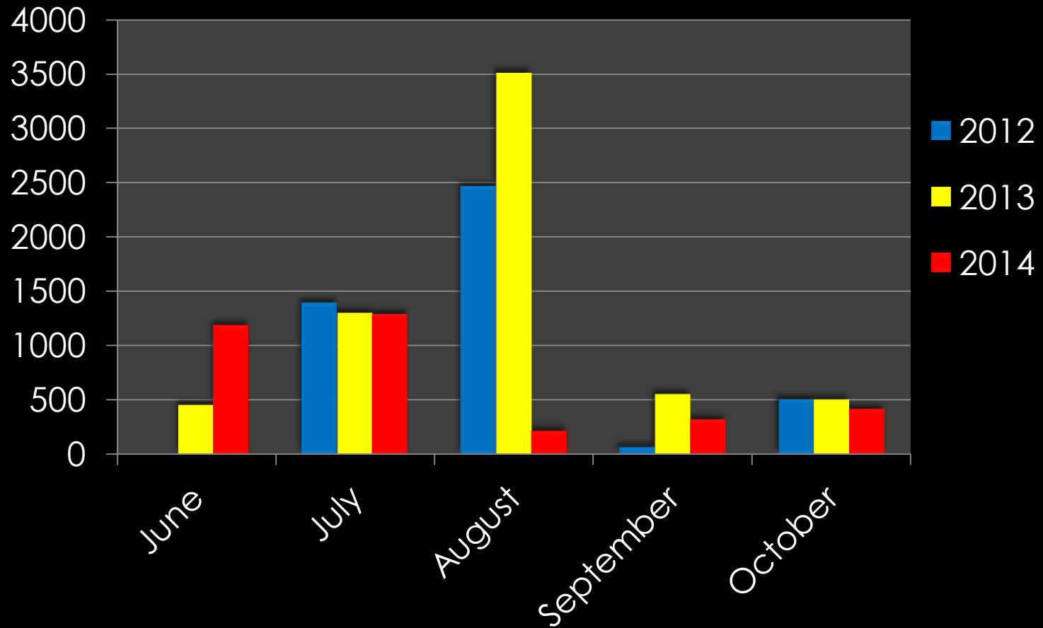
Comparison of Rainfall From 2012-2014
